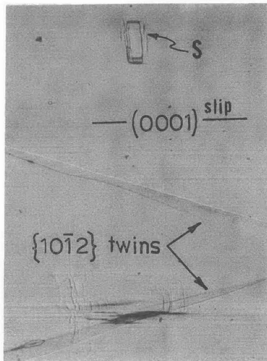
Fig. 3 - Optical Photomicrograph Showing (0001) Slip Lines, \{10\bar{1}2\} Twins and Rectangular Markings at S on (1120) Surface of Crystal ISR-10 Shown in Figure 1. Mag. 240X
